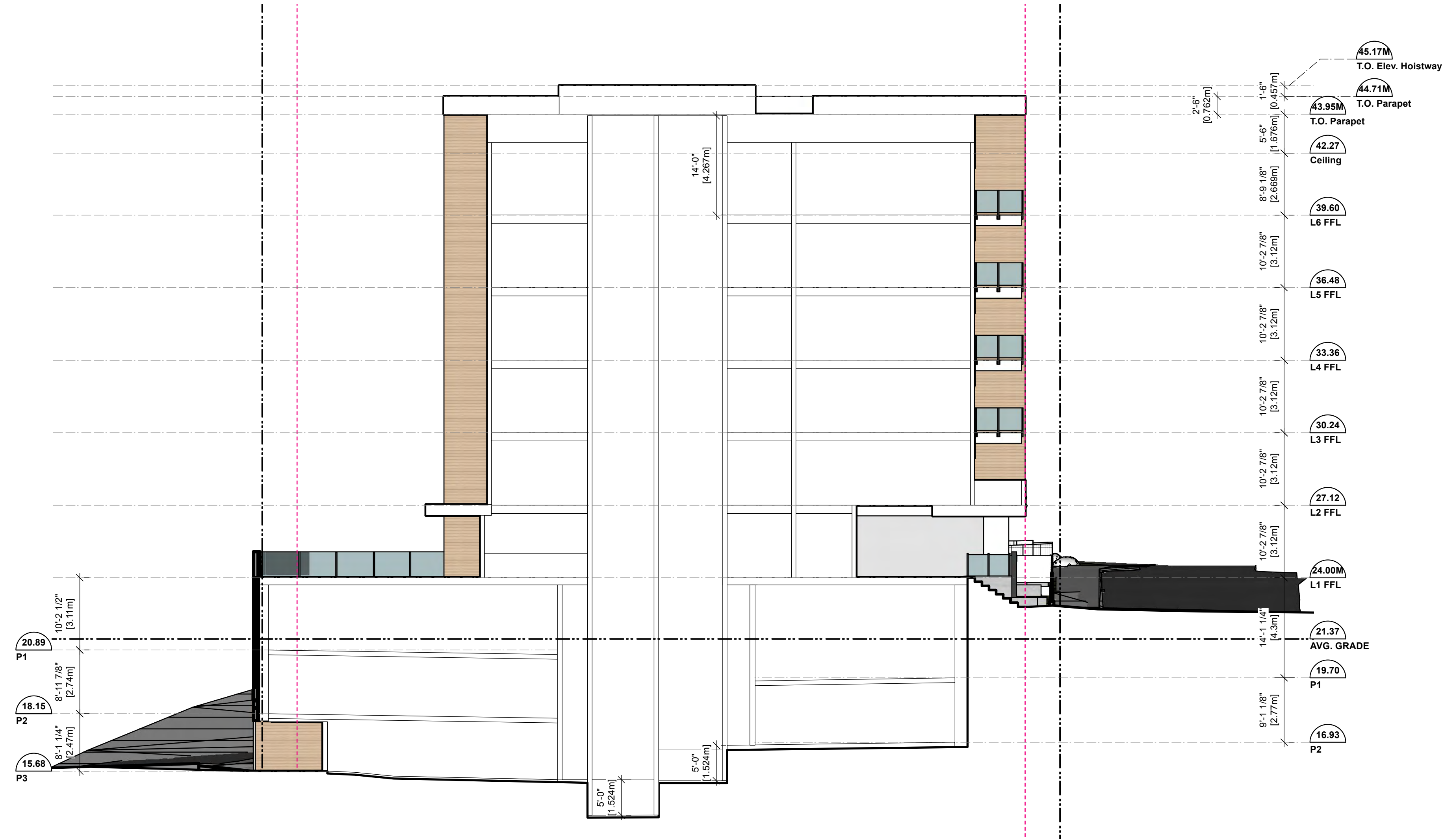
1 Site Section 1 A401 Scale: 3/32" = 1'-0"
